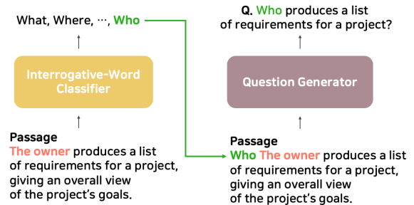
Figure 1: High-level overview of the proposed model.
